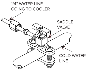
PERMANENT CONNECTION
